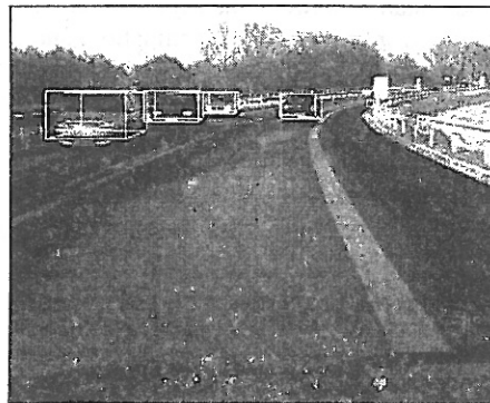
Fig. 11: Perspective view of object cuboids painted over the image
